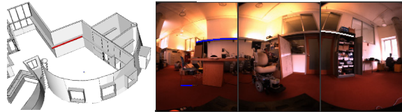
Figure 17. Putative correspondence determined by INIT-SEGMENT-EDGE. The algorithm determines the highest-scoring matches for the model segment (in red on the left) among the observed image edges. The three best candidates are displayed on the right. The correct match appears in blue on the left-hand side.
