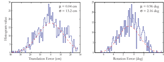
Figure 16. Position and orientation accuracy with respect to ground truth. (Gaussian fit shown as red dashed line).
